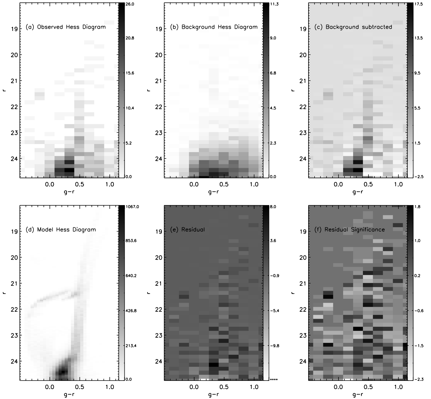
Figure 10. Comparison of the data with our best StarFISH model fit. Pixel bins are 0.15 mag along the color and magnitude axis (except for panel (d), where the bins are 0.05 mag), as used in our StarFISH fits. The grayscale for each Hess diagram is in units of stars per pixel, except for panel (f), which has been scaled by the uncertainty associated with each pixel. (a) The observed Hess diagram of Leo IV within the half-light radius. (b) The background Hess diagram, which was fit along with the theoretical isochrones. (c) The background-subtracted Hess diagram. (d) The best model CMD derived by StarFISH (with no background component), in bins of 0.05 mag in order to show the details of the model. (e) Residuals after subtracting a random realization of the StarFISH model from the data. (f) The residual from (e), scaled by the expected Poisson scatter in the bin. The most significant residuals are associated with the mismatch of the BHB between model and data.
