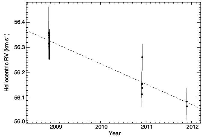
Figure 3. Gl 86 CSHELL RVs after subtracting the planet-induced modulation. The dashed line is a linear fit to the residuals of -0.22 \text{ m s}^{-1} \text{day}^{-1} . A similar long-term trend was presented by Queloz et al. (2000) and indicates the presence of a second, more distant, companion.
