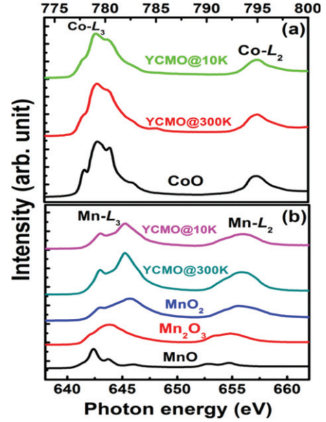
Fig. 2: (Colour on-line) XAS of YCMO at the (a) Co- L_{2,3} and (b) Mn- L_{2,3} edges at 10 K and 300 K with references of \text{Co}^{2+}\text{O} , \text{Mn}^{2+}\text{O} , \text{Mn}_2^{3+}\text{O}_3 and \text{Mn}^{4+}\text{O}_2 spectra.
