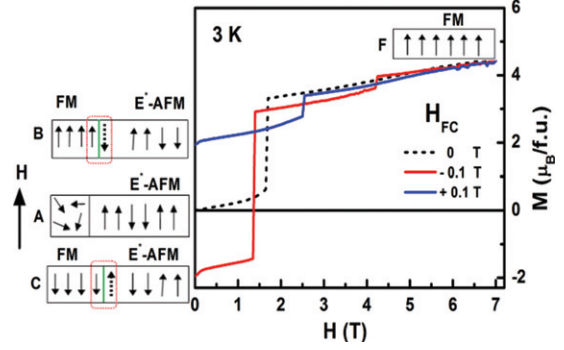
Fig. 5: (Colour on-line) Schematic representation of the resultant interface spin configuration to illustrate the initial and final magnetic states after cooling the system under 0 T and \pm 0.1 T.
