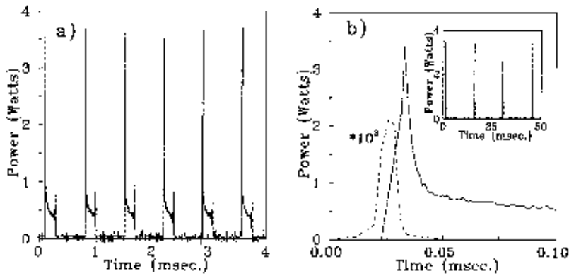
Fig. 4. – a ) Passive Q-switching pulses of LSA for i = 8 mA, without injection. b ) Single pulse response of LSA (solid line) for a small injected signal (dashed line) for i = 4.5 mA. The vertical scale for the injected signal is in mW. Inset: sequence of pulses due to injection. The after pulse plateaux at roughly 0.75 W lasts for a time of about 0.2 ms before the zero state is recovered. The repetition frequency (about 50 Hz, see text) is imposed by SM and C.
