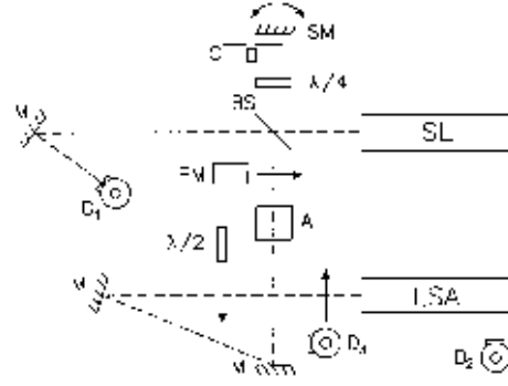
Fig. 3. – Experimental setup. LSA: CO 2 laser with an SF 6 saturable absorber; SL: stabilized CO 2 laser; M: mirrors; SM: scanning mirror; BS: 50 % beam splitter; PM: power meter; A: variable attenuator; D 1 , D 2 , D 3 : fast HgCdTe detectors; \lambda/2 : half-wave plate; \lambda/4 : quarter-wave plate; C: rotating chopper wheel.
