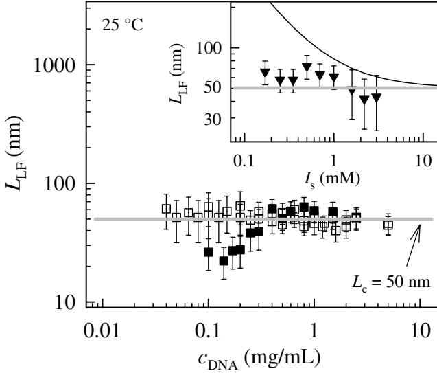
Fig. 3: Main panel: characteristic length of the LF mode ( L_{LF} ) for pure water short-fragment DNA solutions (open squares) and for short-fragment DNA solutions with added salt I_s = 1 mM (full squares) as a function of the DNA concentration ( c_{DNA} ). The full line denotes the contour length L_c \approx 500 Å. Inset: L_{LF} for short-fragment DNA solutions with varying ionic strength of added salt for c_{DNA} = 0.5 mg/mL (full triangles). The grey and full lines denote the contour length of studied short-fragment DNA and the persistence length as predicted by the OSF theory, respectively (ref. [6]).
