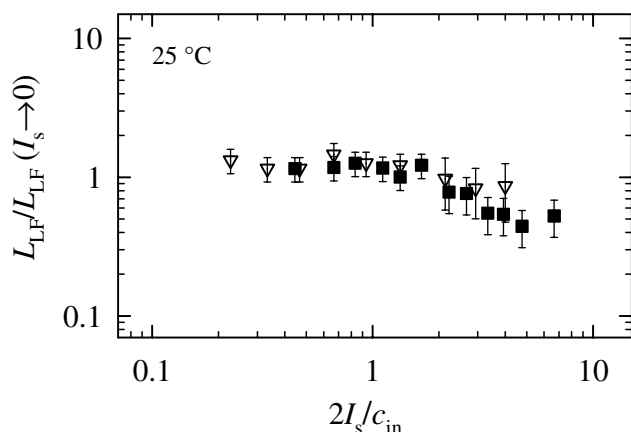
Fig. 4: Characteristic length of the LF mode ( L_{LF} ) normalized with the value in pure water solutions L_{LF}(I_s \rightarrow 0) \approx L_c vs. added-salt concentration normalized by the concentration of intrinsic counterions ( 2I_s/c_{in} ). Data are for one representative DNA concentration c_{DNA} = 0.5 mg/mL and varying I_s (open triangles) and for I_s = 1 mM and varying DNA concentrations (full squares).
