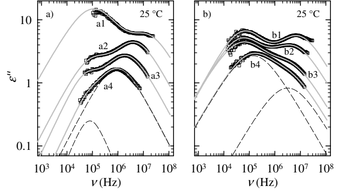
Fig. 1: Double logarithmic plot of the frequency dependence of the imaginary part of the dielectric function ( \epsilon'' ) at T = 25^\circ\text{C} of a) pure water 146 bp DNA solutions (for DNA concentrations a1–a4 (5, 0.5, 0.15, 0.05 mg/mL)) and b) 146 bp DNA solutions with added salt I_s = 1 mM (for DNA concentrations b1–b4 (1.5, 0.8, 0.4, 0.3 mg/mL)). The full lines are fits to the sum of two Cole-Cole forms (see text); the dashed lines represent the single form.
