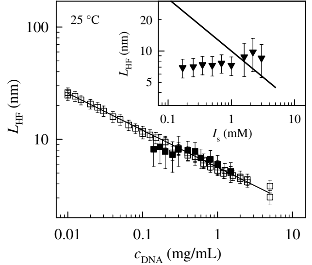
Fig. 2: Main panel: characteristic length of the HF mode ( L_{\text{HF}} ) for pure water short-fragment DNA solutions (open squares) and for short-fragment DNA solutions with added salt I_s = 1 \text{ mM} (full squares) as a function of DNA concentration ( c_{\text{DNA}} ). The full line is a fit to the power law L_{\text{HF}} \propto c_{\text{DNA}}^{-0.33} . Inset: L_{\text{HF}} for short-fragment DNA solutions vs. added salt ( I_s ) for c_{\text{DNA}} = 0.5 \text{ mg/mL} (full triangles). The full line denotes the Debye screening length for the investigated range of added salt.
