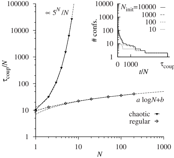
Fig. 2: Chaotic and regular couplings for the random walk in an N -dimensional hypercubic lattice of length L=5 (see eqs. (2) and (3), respectively). The random process for a single random walk is defined by eq. (1) in both cases. Inset: number of configurations vs. time as a function of the number N_{\text{init}} of initial configurations, for N=6 , L=5 for the chaotic coupling. The same realization of the coupling of eq. (3) is used for all runs.
