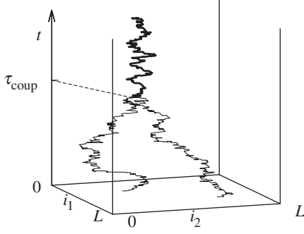
Fig. 1: Coupling of two random walks in a periodic N -dimensional hypercubic lattice of length L . After the time \tau_{\text{coup}} , the two random walks evolve identically. The chaotic coupling of eq. (2) is shown. For the regular coupling of eq. (3), the displacement at time t is in the same direction k , and it is a function of i_k only.
