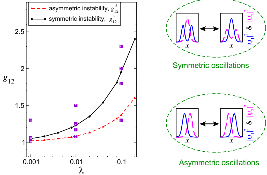
Figure 2. Left: the dynamical ‘phase diagram’ showing the critical values of g_{12} for the onset of the two types of modulation instability versus the trap strength \lambda . The instability lines are shown as straight lines joining numerically determined values. Right bottom: spatially asymmetric (left–right–left) oscillation mode, shown schematically through density profiles of the two components at two instants of an oscillation period. This type of mode is persistent everywhere above the g_{12}^a line. Right top: spatially symmetric (in–out–in) oscillation mode, shown schematically through density profiles of the two components at two instants of an oscillation period. This type of mode is persistent only above the higher g_{12}^s line. The spatially symmetric instability ( g_{12}^s line) is the one relevant for experimental situations with symmetric traps. Squares mark values used in the dynamical simulations of figures 3 and 4 (table 1).
