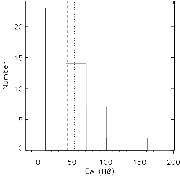
Fig. 1 The distribution of H\beta EWs in our sample. The dashed line and dotted line represent the median and average EWs of 42.9 Å and 53.5 Å, respectively.
