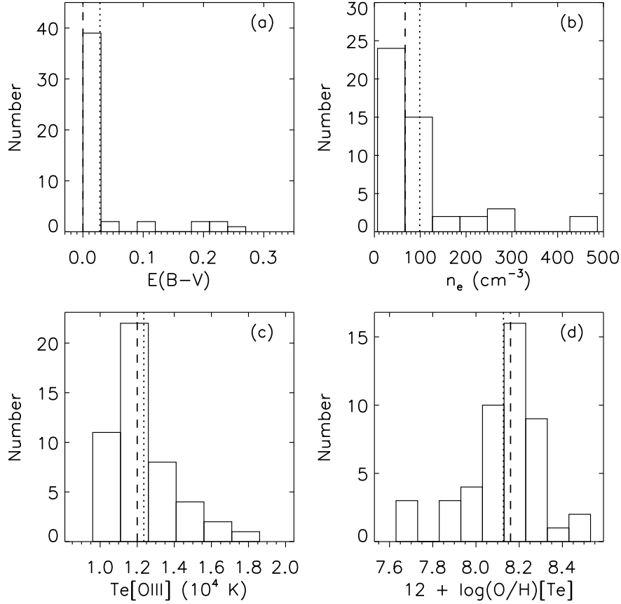
Fig. 4 The distributions of color excesses, electron densities, electron temperatures and oxygen abundances for our sample galaxies. The dashed lines represent median values of these parameters, 0.00 mag, 67.0 \text{ cm}^{-3} , 1.20 \times 10^4 \text{ K} and 8.16, respectively. The dotted lines represent the average values of 0.03 mag, 98.9 \text{ cm}^{-3} , 1.24 \times 10^4 \text{ K} and 8.13, respectively.
