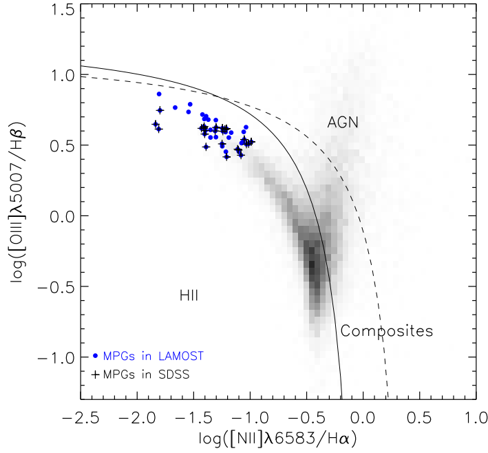
Fig. 2 BPT diagram for our metal-poor galaxy (MPG) sample and all the LAMOST galaxies. The blue dots represent our final sample galaxies. The black crosses represent these objects in our final sample that have also been spectrally detected with SDSS. The grayscale 2D histogram shows the number density of LAMOST galaxies. The solid and dashed lines are the demarcation curves between star forming galaxies and AGNs defined by Kauffmann et al. (2003) and Kewley et al. (2001), respectively.
