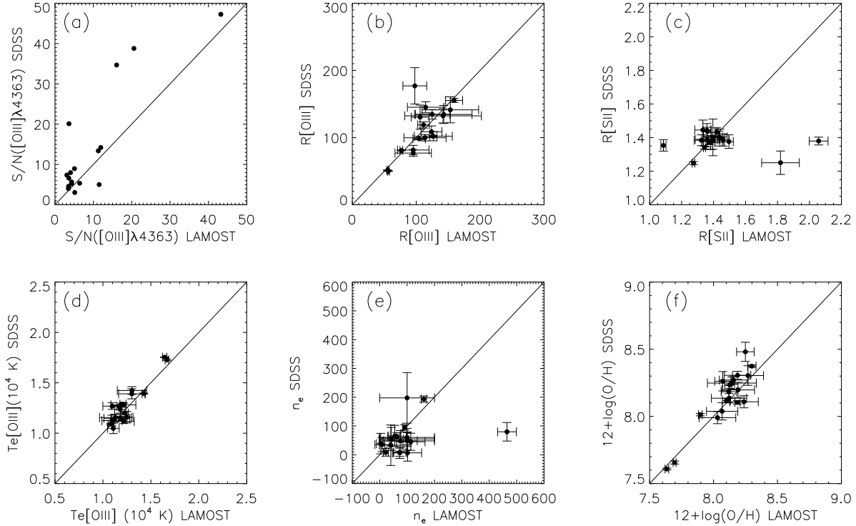
Fig. 6 Comparisons of S/N values for weak [\text{O III}]\lambda 4363 lines, [\text{O III}] line flux ratios ( R[\text{O III}] = [\text{O III}]\lambda\lambda 4959, 5007/[\text{O III}]\lambda 4363 ), [\text{S II}] line flux ratios ( R[\text{S II}] = [\text{S II}]\lambda 6717/[\text{S II}]\lambda 6731 ), electron temperatures, electron densities and oxygen abundances derived from LAMOST spectra and from SDSS spectra for 19 galaxies in our sample. The solid lines indicate equality between the LAMOST and SDSS measurements.
