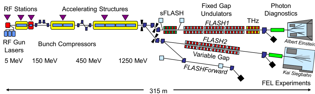
Figure 1. Layout of the FLASH facility.
