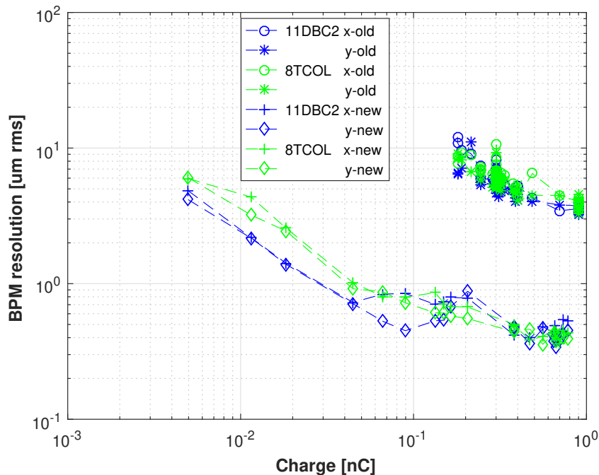
Figure 3. Strip-line BPM resolution (old/new).
