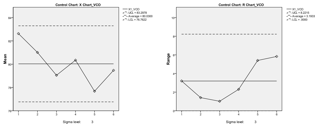
Figure 3. X and R Control Chart on VCO Biodiesel
