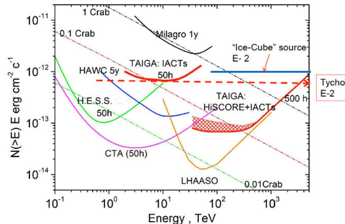
Figure 4. The TAIGA-HiSCORE and TAIGA-IACT point source sensitivity (preliminary) in comparison to other experiments.
