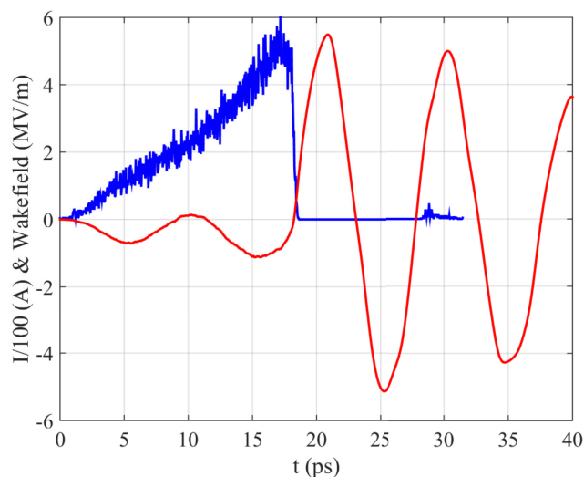
Figure 4. Current profiles at the entrance to the structure (blue). Wakefield calculated by the convolution of the current profile and the wake function (red).
