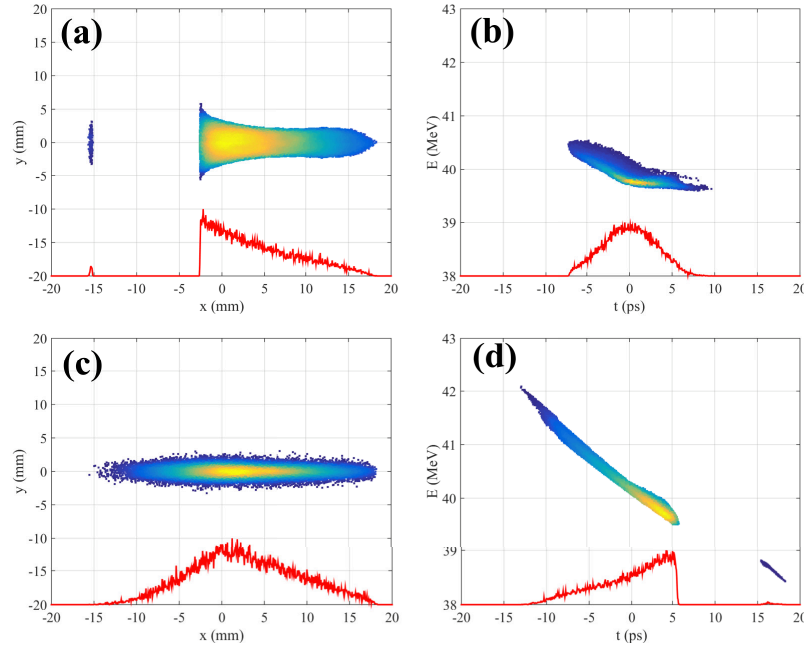
Figure 2. (a) x-y projection and (b) longitudinal phase space after the mask. (c) x-y projection and (d) longitudinal phase space after the second EEX beamline. Red curves are projections to the x-axis (i.e. horizontal profile or temporal profile)
