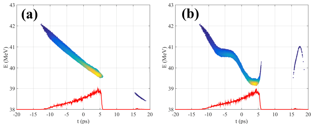
Figure 5. Longitudinal phase space before (a) and after (b) the CWFA structure. Red curves are temporal profiles.
