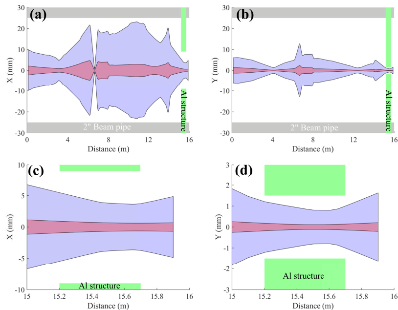
Figure 3. Horizontal (a) and vertical beam (b) envelope along the double EEX beamline. The red envelopes show the sigma for x and y, and the blue envelopes show the full size of the beam for x and y. (c) and (d) show the beam envelopes near the structure.
