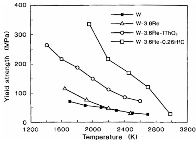
Figure 17. Yield strength of tungsten and some of its high-strength alloys.
