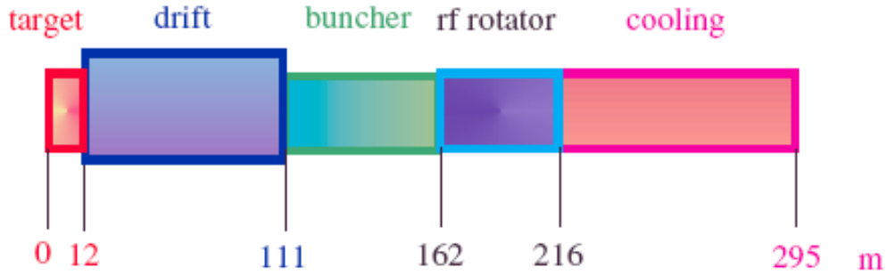
Figure 31. Schematic layout of ISS baseline front end.
