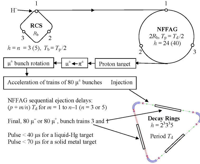
Figure 2. Bunch patterns ( n = 3 ) for the proton driver and decay rings. This example assumes triangular decay rings.
