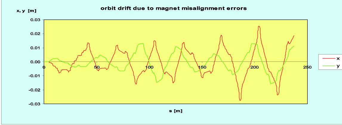
Figure 51. Orbit deviation due to magnet misalignment errors.
