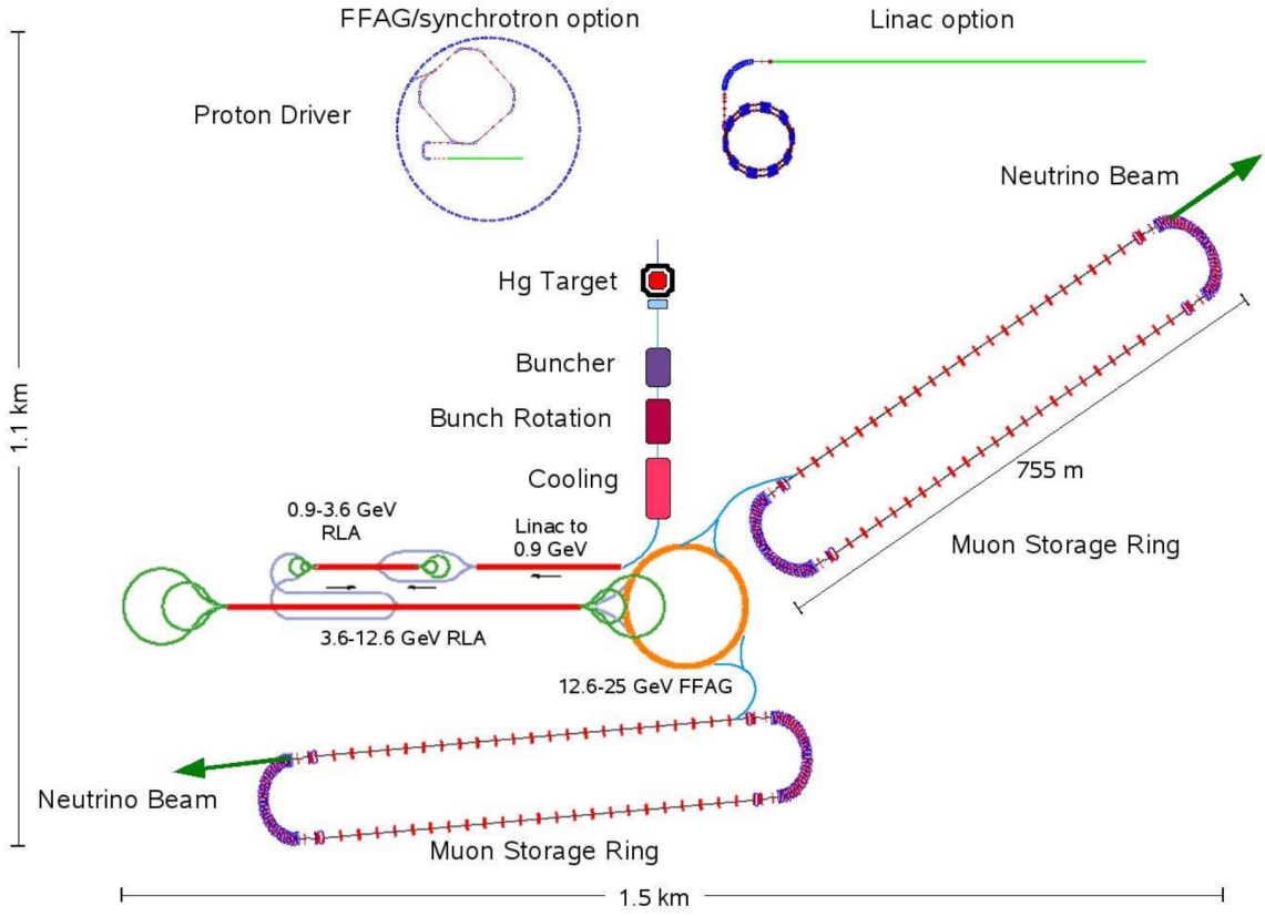
Figure 62. Overall Neutrino Factory baseline configuration.
