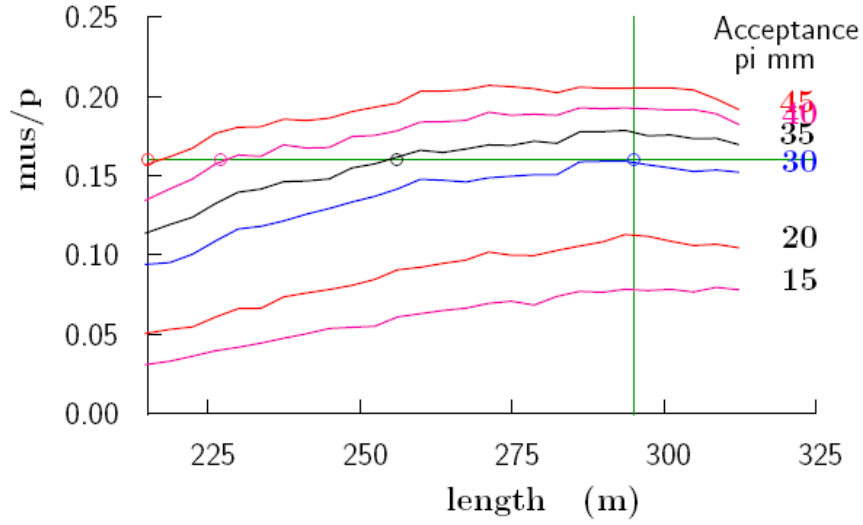
Figure 30. Accepted number of muons per proton as a function of distance along the cooling channel for various assumed downstream accelerator transverse acceptances. The cooling channel begins at 216 m in the length coordinate plotted.
