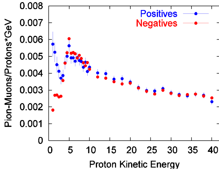
Figure 11. Calculated production efficiency for a carbon target. The yield per proton and per GeV is lower than for a mercury target and peaks at a lower energy.
