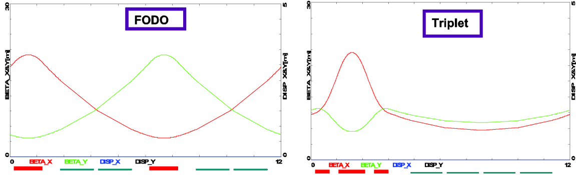
Figure 43. Comparison of FODO and triplet focusing structures. Both designs use the same cell length (12 m) and betatron phase advance per cell ( 90^\circ ).
