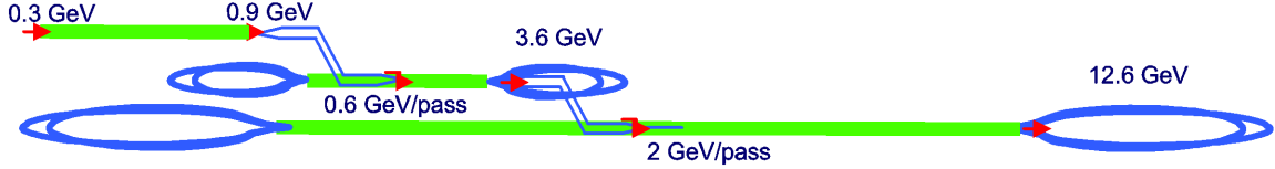
Figure 41. Layout of two-step dogbone RLA complex. For compactness, all three subsystems (pre-accelerator, dogbone I and dogbone II) are stacked up vertically; \mu^\pm beam transfer between the accelerator components is facilitated by the vertical double chicane (see text).
