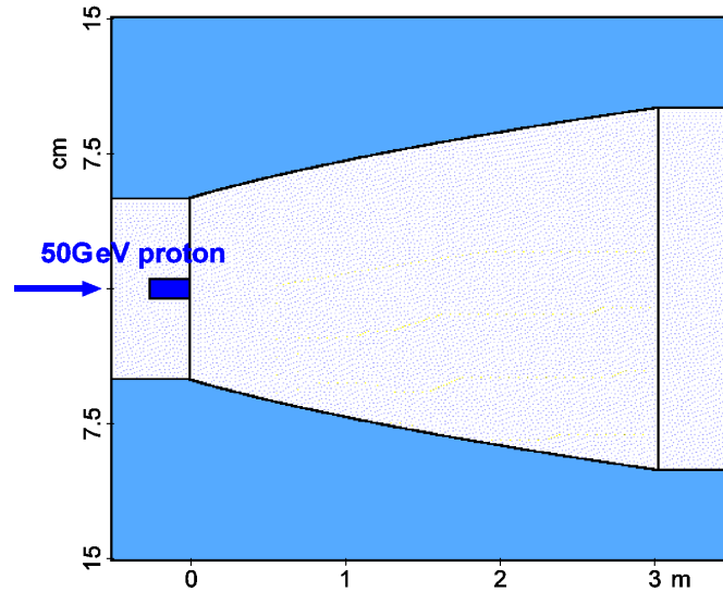
Figure 20. Capture system from ref. [32], comprising a 20 T solenoid followed by a rapid taper to 5 T.
