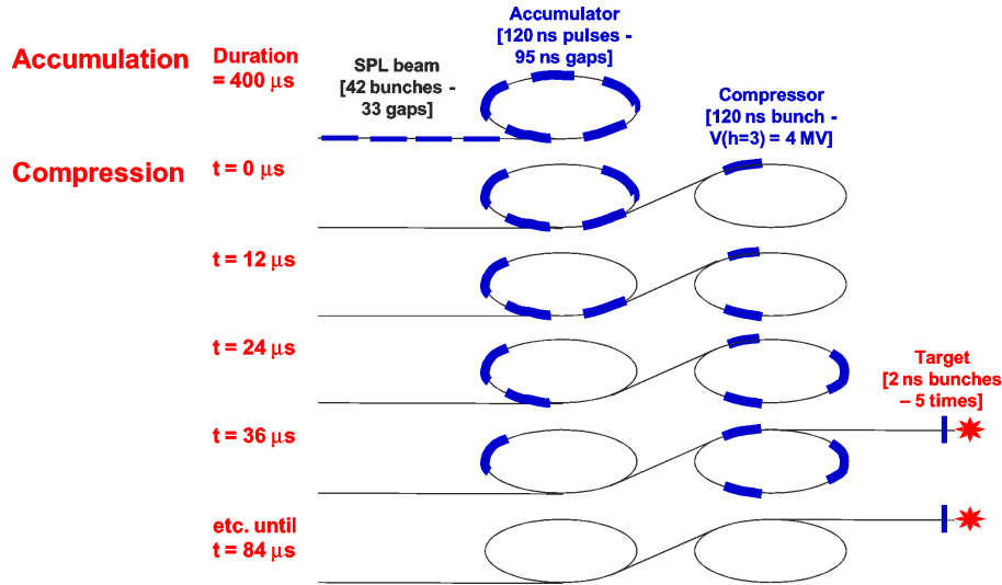
Figure 9. Accumulation and compression scheme for linac-based proton driver.
