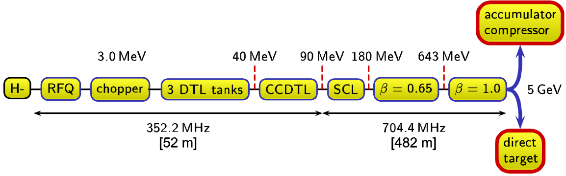
Figure 8. SPL block diagram.
