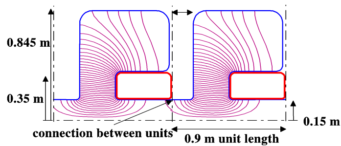
Figure 24. 88 MHz vacuum cavity with integrated solenoids.
