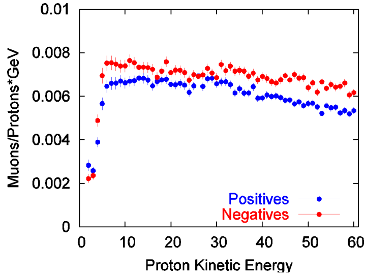
Figure 10. Calculated production efficiency of positive and negative muons at the end of the Study 2a cooling channel, per proton and per GeV of proton beam energy, for a mercury-jet target. Although the curves are rather flat, an optimum energy, roughly 10 GeV, is discernible. Below about 5 GeV, the calculations show an abrupt fall-off in production. Above 10 GeV the fall-off is small but, from the muon production perspective, there is no benefit to increasing the beam energy beyond 10 GeV.
