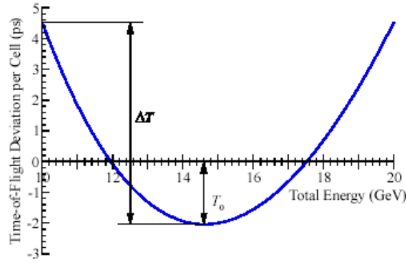
Figure 52. Time-of-flight as a function of energy in a linear, non-scaling FFAG cell.
