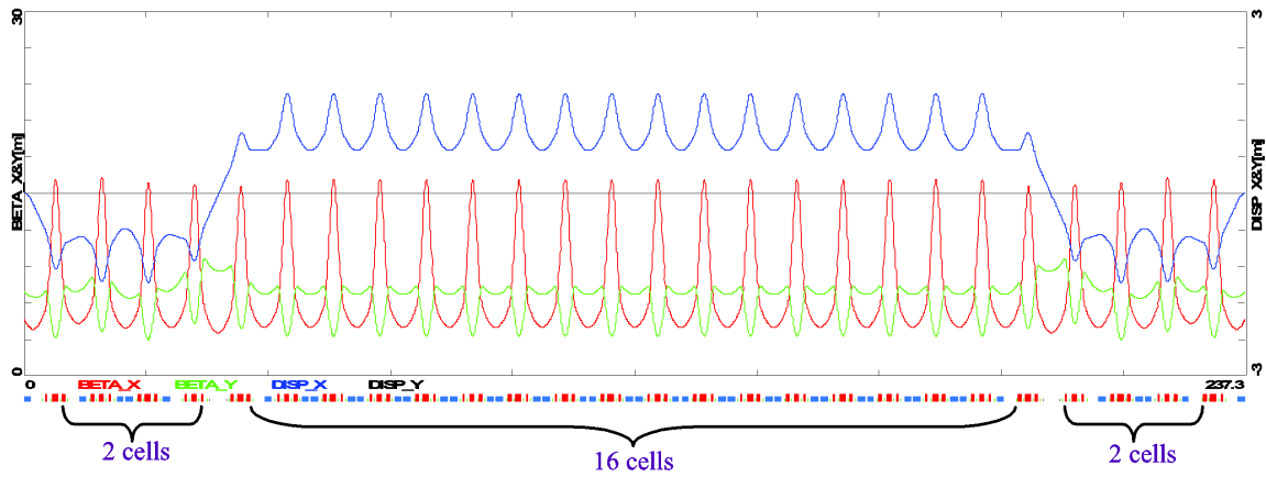
Figure 48. Droplet arc optics, showing uniform periodicity of beta functions and dispersion.
