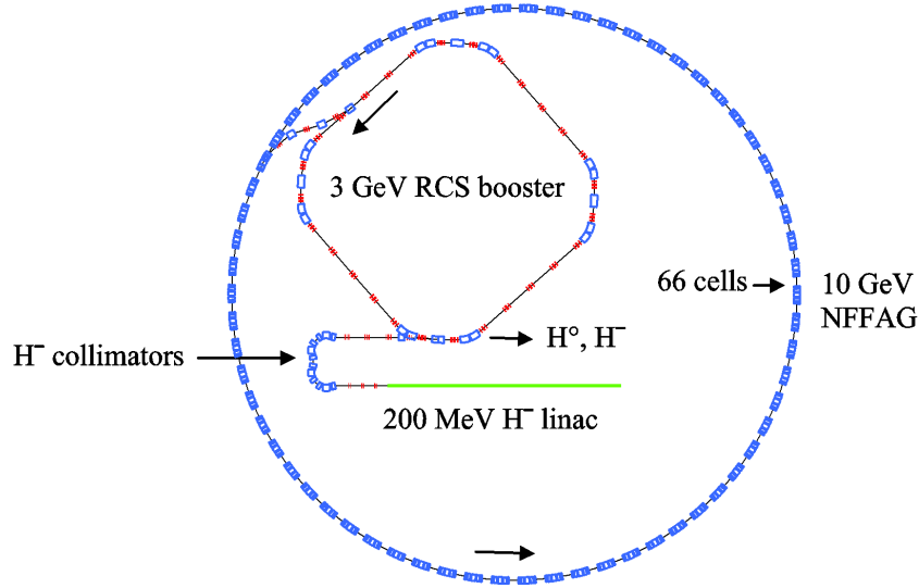
Figure 6. Schematic layout drawing of the linac, booster and NFFAG of the proton driver.
