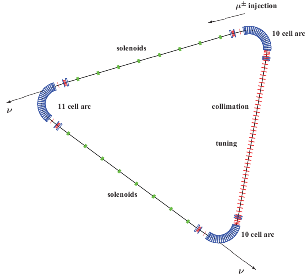
Figure 60. Schematic layout for a 52.8^\circ apex angle, isosceles triangle, muon decay ring.
