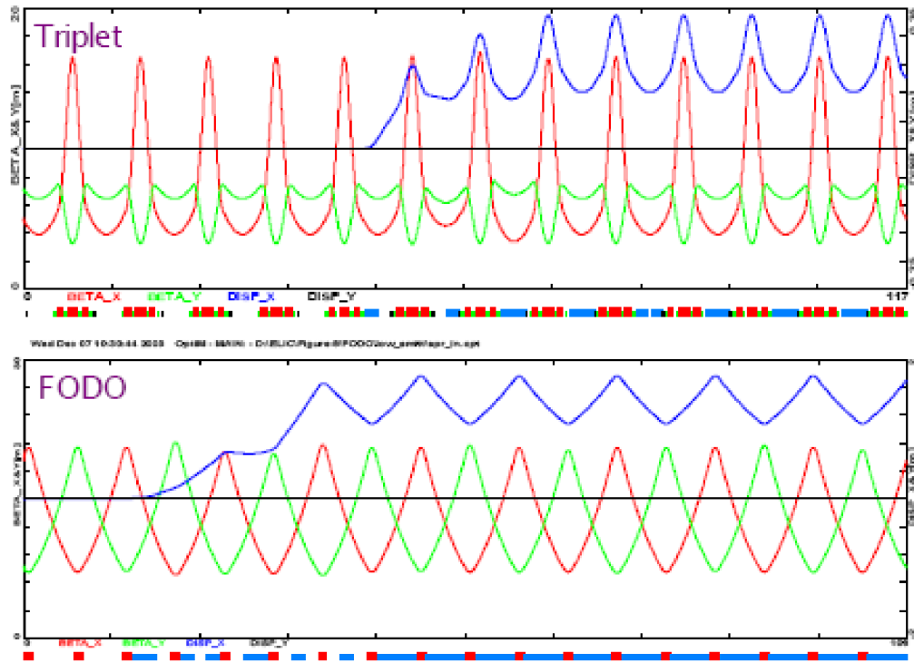
Figure 49. Spreader optics showing uniform periodicity of beta functions and dispersion. These optics apply to the triplet design (top) or the FODO design (bottom).
