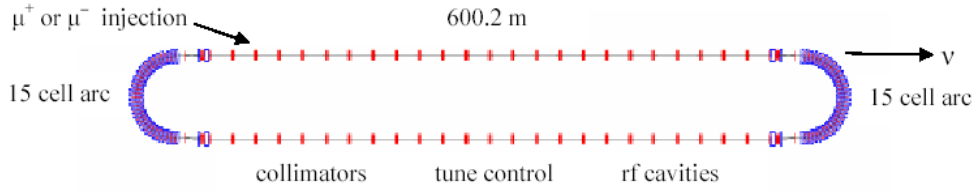
Figure 58. Schematic layout for a racetrack-shaped muon decay ring.
