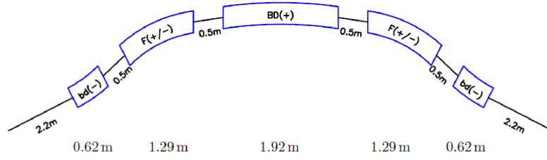
Figure 5. A single lattice cell of the 50 Hz, 4 MW, 10 GeV, NFFAG proton driver ring.
