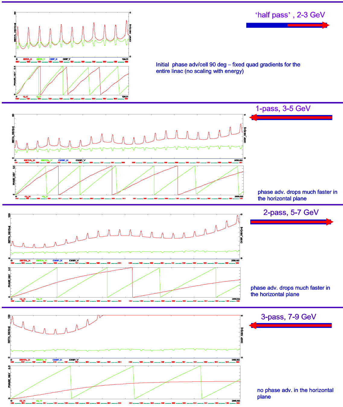
Figure 44. Triplet based multi-pass linac optics. Quadrupoles in all cells are set to the same gradient, corresponding to 90^\circ phase advance per cell at 2 GeV. Intrinsic to triplet focusing, the asymmetry between the horizontal and vertical planes (middle quadrupole focuses horizontally, outer quadrupoles focus vertically) manifests itself via a rapid phase advance loss in the horizontal plane for higher passes; already by the third pass horizontal focusing is almost lost, resulting in catastrophic beam blow-up.
