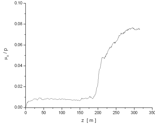
Figure 32. Number of muons per incident proton accepted by the downstream acceleration system vs. longitudinal position along the ISS front end. The cooling channel begins at 216 m in this plot. Note that some increase in accepted muons takes place in the phase rotation section upstream of the cooling channel, where more particles are moved into the energy acceptance of the acceleration system.
