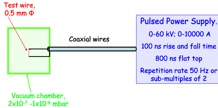
Figure 13. Schematic diagram of the test wire and power supply.
