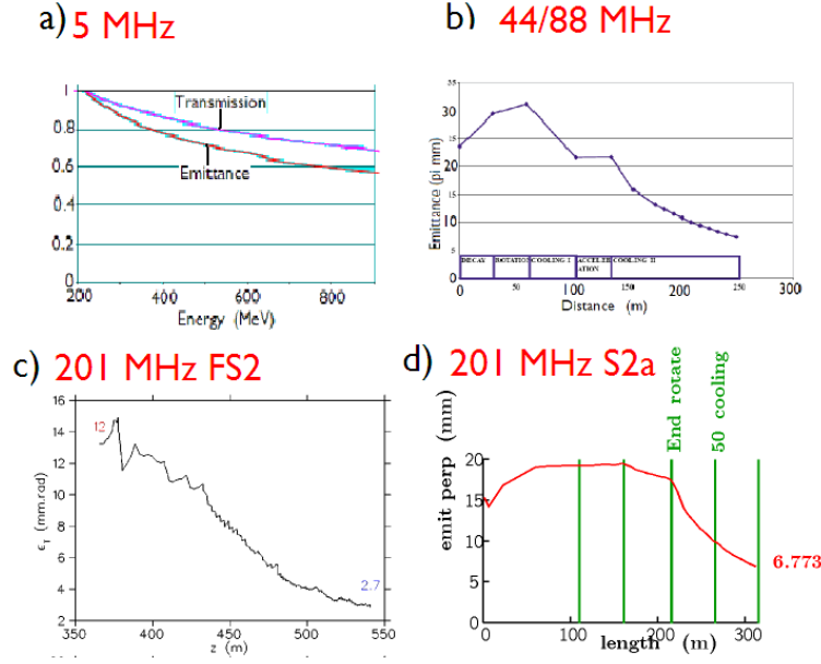
Figure 29. Emittances vs. distance along cooling channel: a) 5 MHz in an FFAG; b) 44 and 88 MHz tapered system; c) Study 2 tapered system at 201 MHz; d) Study 2a non-tapered system. In a), “distance” is represented in units of the beam energy after some number of turns in the ring.
