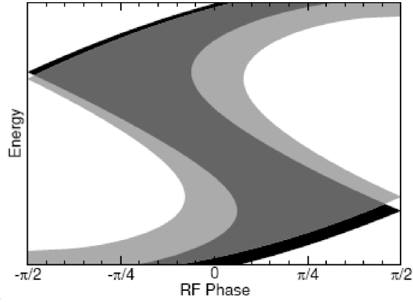
Figure 54. Phase space channel for low amplitude particles (black) and high amplitude particles (light grey). The overlap region is dark grey. Particles start at low energy (bottom) and are accelerated to high energy (top).
