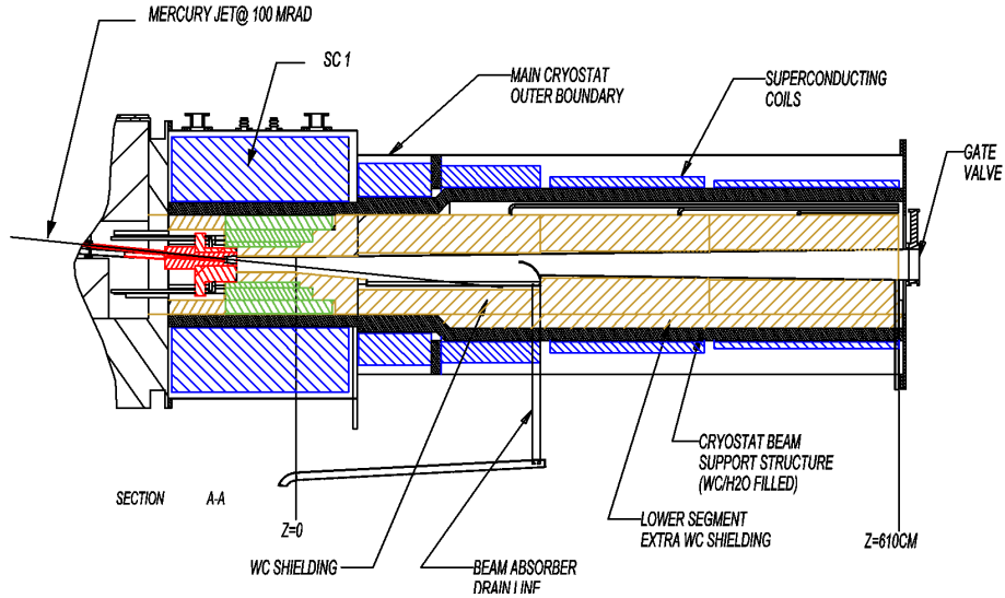
Figure 18. Baseline ISS target system. The solenoidal field at the target position is 20 T. The downstream coils begin the process of adiabatically tapering the field to 1.75 T for further transport.
