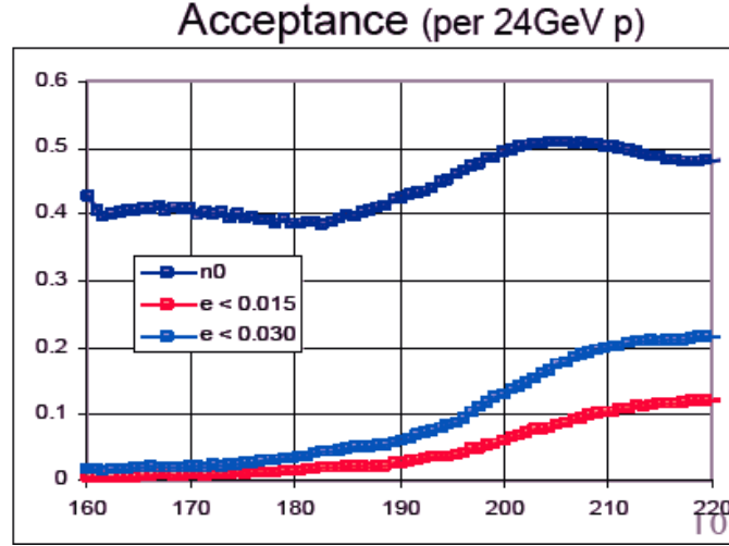
Figure 36. Accepted number of muons per incident proton as a function of distance in the gas-filled cooling channel. The upper (dark blue) curve is the total number of \mu/p , the middle (light blue) curve is \mu/p into the ISS acceptance, and the bottom (red) curve is \mu/p into the Study 2 acceptance.
