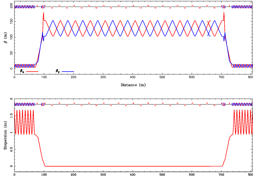
Figure 59. Betatron (top) and dispersion (bottom) functions in a racetrack ring.
