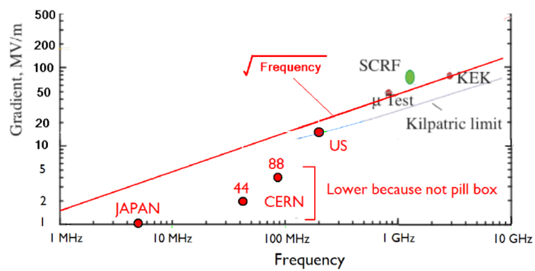
Figure 26. Gradients vs. frequency.
