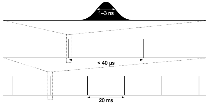
Figure 1. Proton bunch structure. The top picture represents a single proton micro-bunch, the middle picture shows the spacing of three such micro-bunches that hit the production target in one proton driver cycle, and the bottom picture shows the overall 50 Hz repetition rate of the proton driver.
