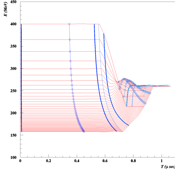
Figure 34. Energy of a set of test particles as a function of time in the phase rotation channel.
