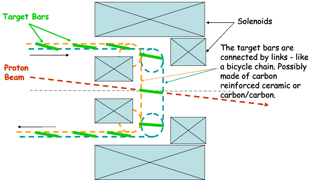
Figure 12. Schematic diagram of a solid target scenario.
