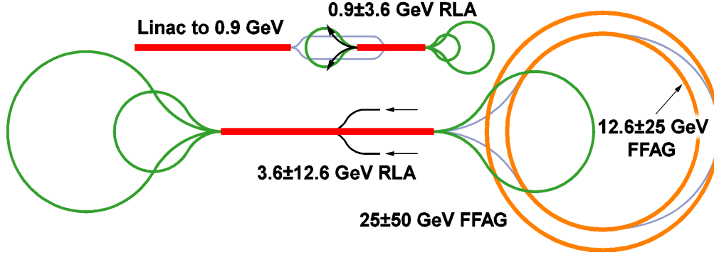
Figure 37. Layout of the acceleration system.
