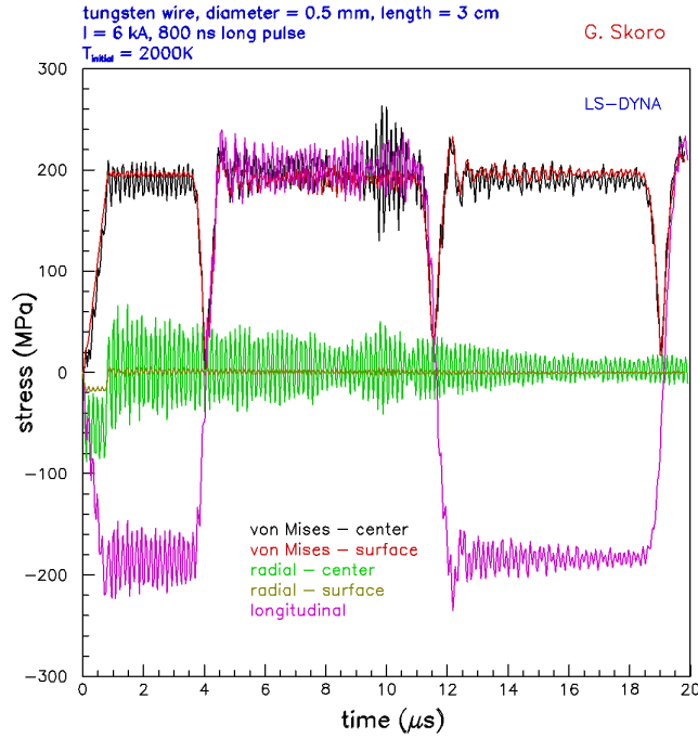
Figure 16. Typical radial stress in the tungsten wire from thermal and Lorentz forces.
