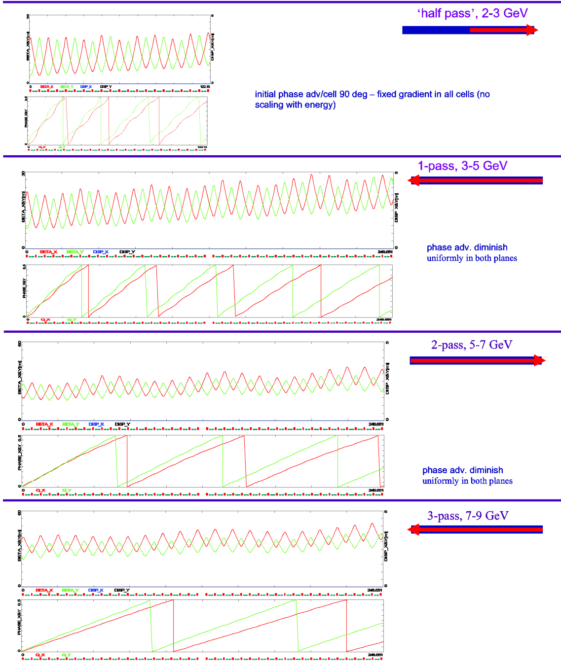
Figure 45. FODO based multi-pass linac optics for passes 1–3. Quadrupoles in all cells are set to the same gradient, corresponding to 90^\circ phase advance per cell at 2 GeV. Intrinsic to the FODO focusing symmetry between the horizontal and vertical planes, the betatron phase advances gradually diminish uniformly in both planes. The resulting linac optics is well balanced in terms of Twiss functions and beam envelopes, and there is sufficient phase advance for up to six passes.
