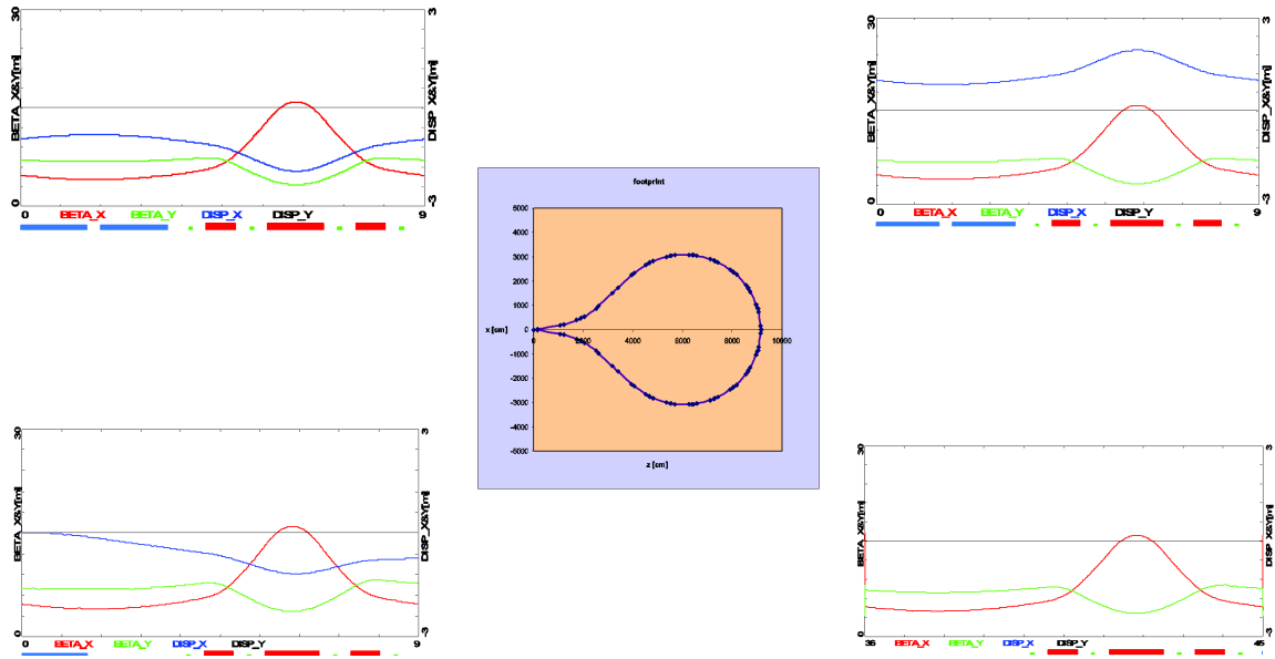
Figure 47. The lattice building blocks: triplet 90^\circ phase advance cells; inward and outward cells, missing dipole empty cells.
