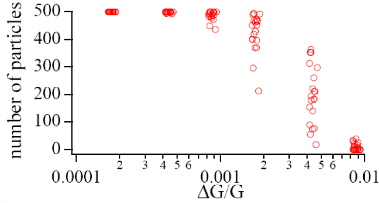
Figure 56. Number of surviving particles as a function of gradient error.
