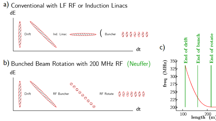
Figure 19. Phase rotation methods: a) conventional; b) Neuffer bunched beam phase rotation. c) Shows frequency vs. distance for the case of Study 2a, a version of b).
