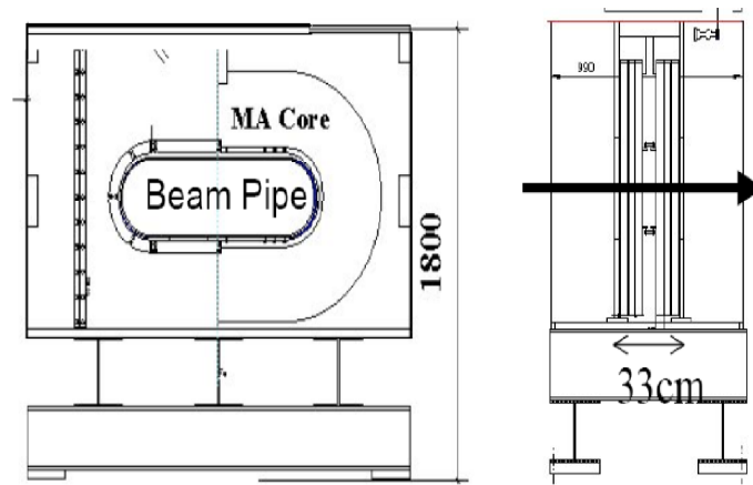
Figure 23. 5 MHz ferrite-loaded cavity for FFAG scheme.
