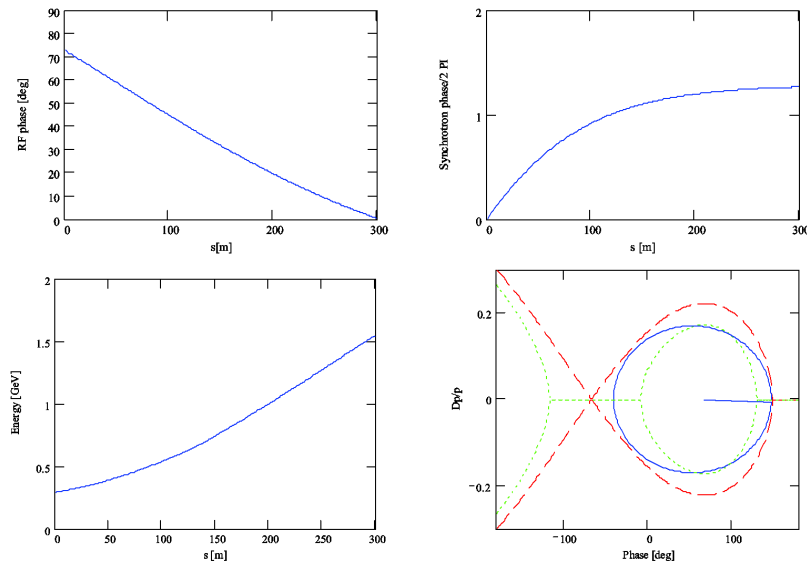
Figure 39. Individual cavity phasing along the linac and the resulting synchrotron motion. The energy profile and the longitudinal beam boundary (solid line) inside a separatrix (dashed line) are shown at the beginning of the linac ( \Delta p/p = \pm 0.17 or \Delta\phi = \pm 92^\circ ).
