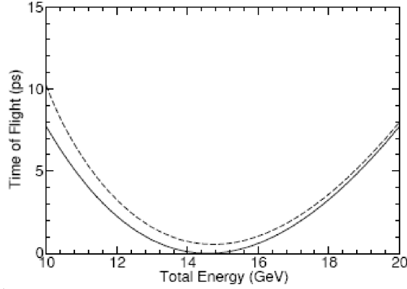
Figure 53. Time-of-flight as a function of energy for zero transverse amplitude (solid) and 30\pi mm-rad (dashed) normalized transverse amplitude (twice the transverse action, normalized).
