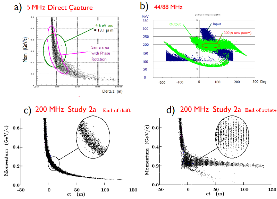
Figure 27. Phase-space plots of phase rotation cases: a) 5 MHz before rotation with captured ellipses without rotation (green), and with rotation (magenta); b) CERN 44 MHz, before (blue) and after (green) rotation with eventual 88 MHz acceptance in red; c) and d) Study 2a before and after rotation.
