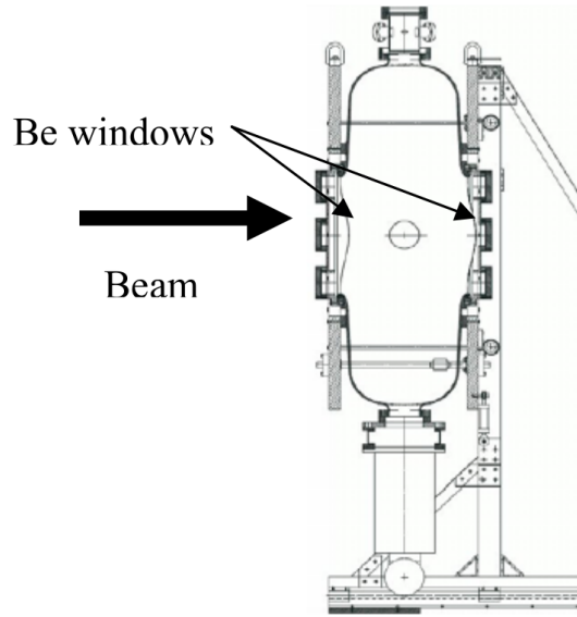
Figure 25. 201 MHz test cavity, showing mounting arrangement. The ports on the entrance and exit faces are for diagnostic purposes. The curved surfaces represent thin Be windows that electrically close the irises.
