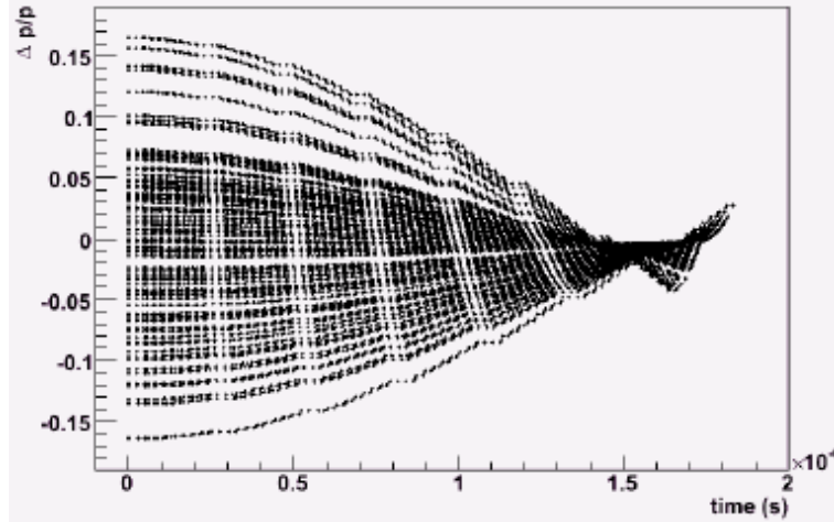
Figure 35. Energy spread of Gaussian beam versus time in the simulation model of PRISM.
