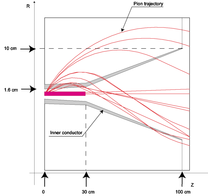
Figure 21. CERN horn capture option.
