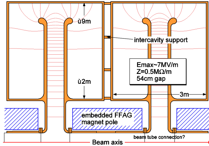
Figure 22. 5 MHz vacuum cavity for FFAG scheme.
