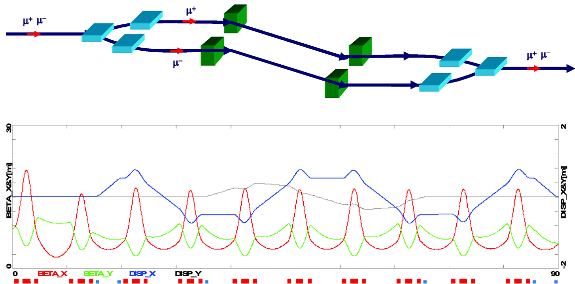
Figure 50. Layout and optics of the injection double chicane.
