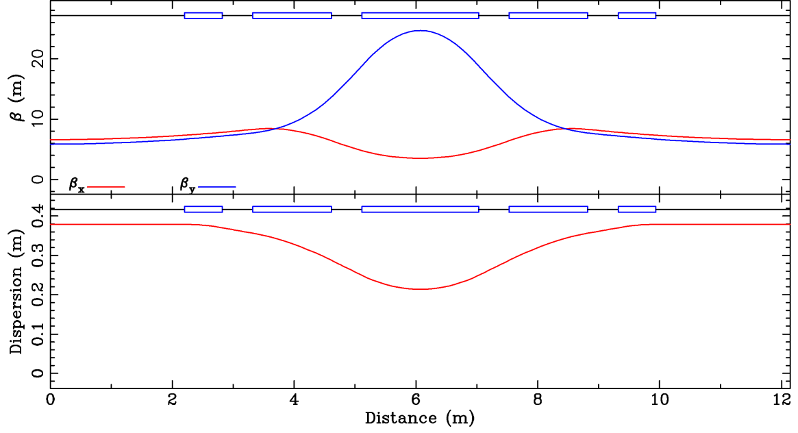
Figure 7. Small amplitude betatron (top) and dispersion (bottom) functions for the NFFAG 10 GeV orbit.
