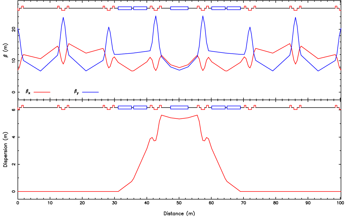
Figure 4. (upper) Betatron functions for the 400.8 m booster synchrotron; (lower) booster dispersion function.
