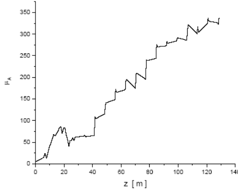
Figure 33. Number of muons in the accelerator acceptance vs. distance along the CERN channel.
