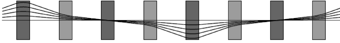
Figure 55. Trajectories in a FODO lattice, demonstrating that path lengths are longer for particles with larger transverse amplitude.
