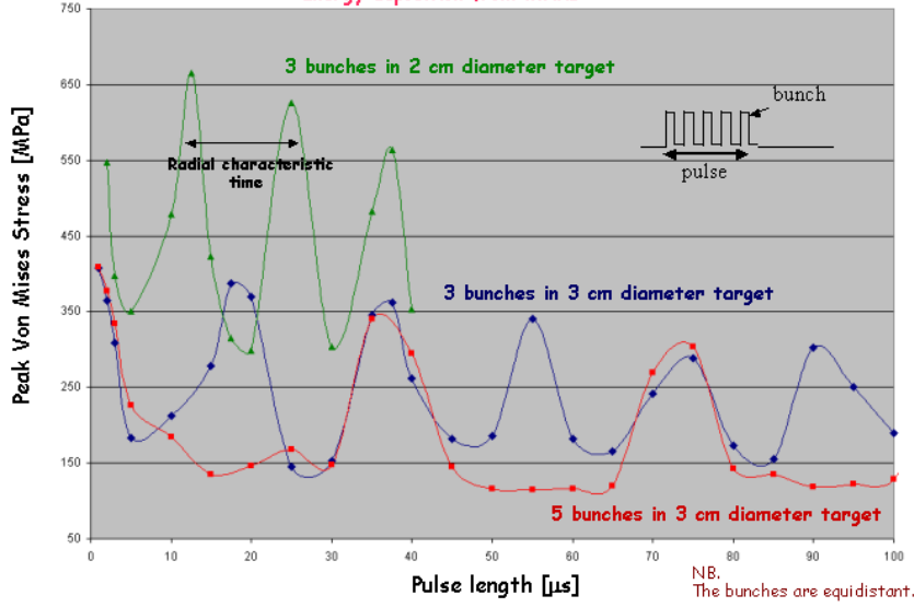
Figure 15. Thermal stress as a function of target diameter, number and spacing of proton bunches in a macro-pulse.
