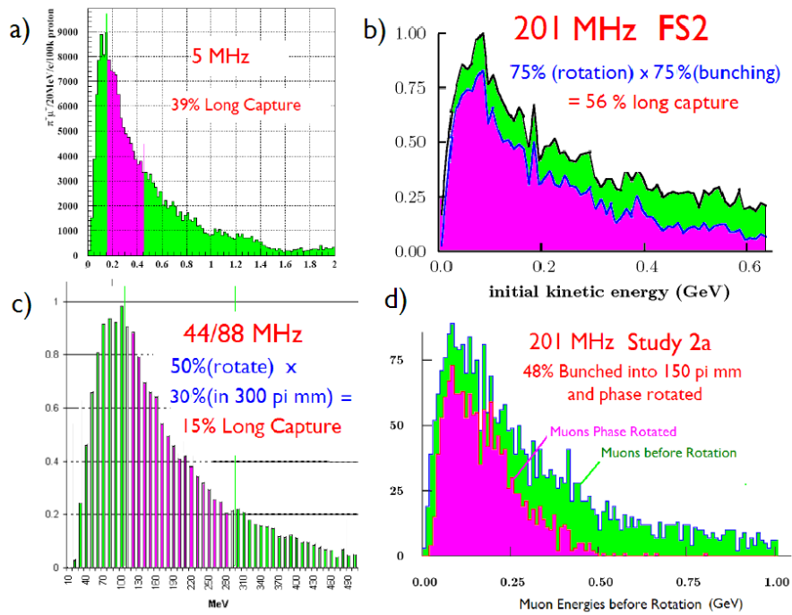
Figure 28. Momentum ranges captured by various phase rotation systems: a) 5 MHz without phase rotation; b) induction linac system; c) 44 MHz rotation; d) 201 MHz bunched beam phase rotation.
