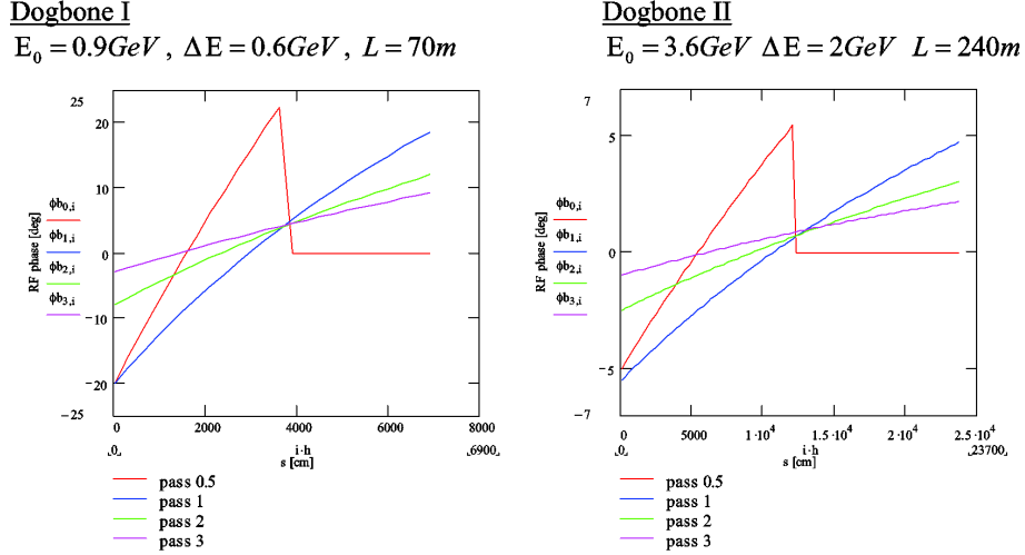
Figure 42. RF phase slippage along the multi-pass linacs; initial ‘gang phases’ for each pass were chosen for optimum longitudinal bunch compression in each linac-arc segment. For dogbone 1, the gang phases were -20^\circ , -20^\circ , -8^\circ , and -3^\circ , respectively, for the four passes through the device; for dogbone 2, the gang phases were -5^\circ , -5.5^\circ , -2.5^\circ , and -1^\circ , respectively, for the four passes.
