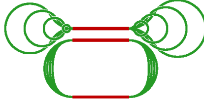
Figure 40. RLA geometries: dogbone layout (above), racetrack layout (below).
