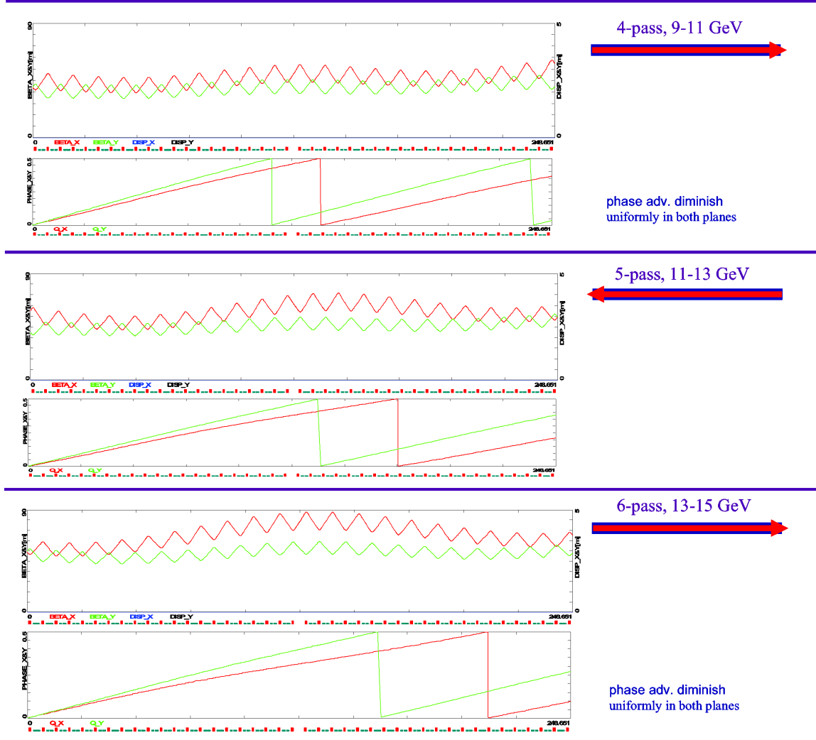
Figure 46. FODO based multi-pass linac optics for passes 4–6. Quadrupoles in all cells are set to the same gradient, corresponding to 90^\circ phase advance per cell at 2 GeV. Intrinsic to the FODO focusing symmetry between the horizontal and vertical planes, the betatron phase advances gradually diminish uniformly in both planes. The resulting linac optics is well balanced in terms of Twiss functions and beam envelopes, and there is sufficient phase advance for up to six passes.
