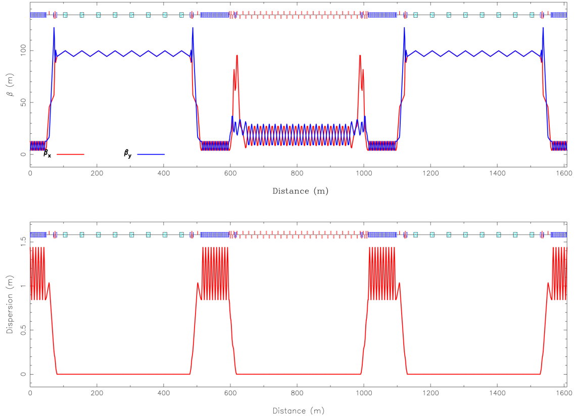
Figure 61. Lattice betatron (top) and dispersion (bottom) functions for the 1608.8 m triangle decay rings.
