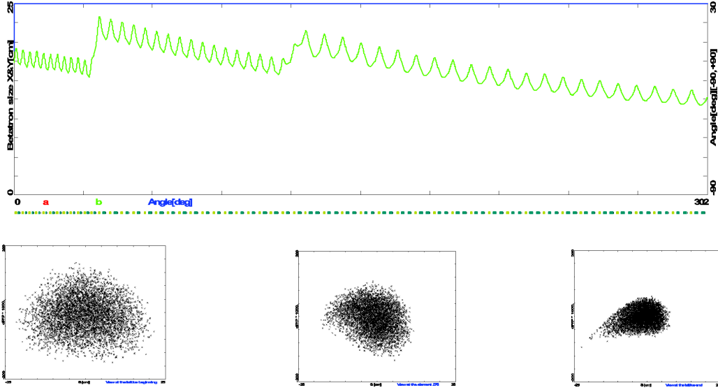
Figure 38. Top, transverse beam envelopes in the pre-accelerator linac, which has uniform periodic focusing with three styles of cryo-modules. Below, longitudinal phase-space: before, halfway through, and at the end of acceleration, as obtained by particle tracking.
