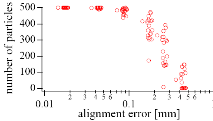
Figure 57. Number of surviving particles as a function of alignment error.
