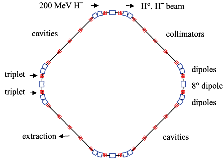
Figure 3. Layout of 50 Hz, 3 GeV booster synchrotron.
