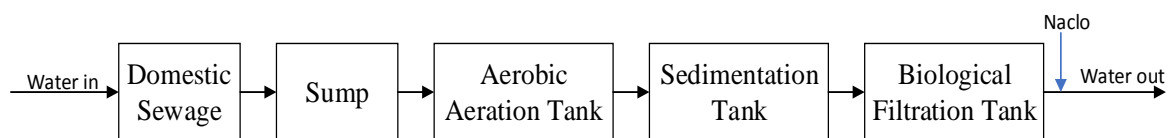
Figure 4. Process flow chart.
