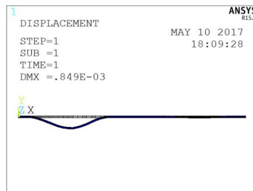
Figure 5: Deformation of longitudinal rod with intermediate support under 'tread pole' conditions
